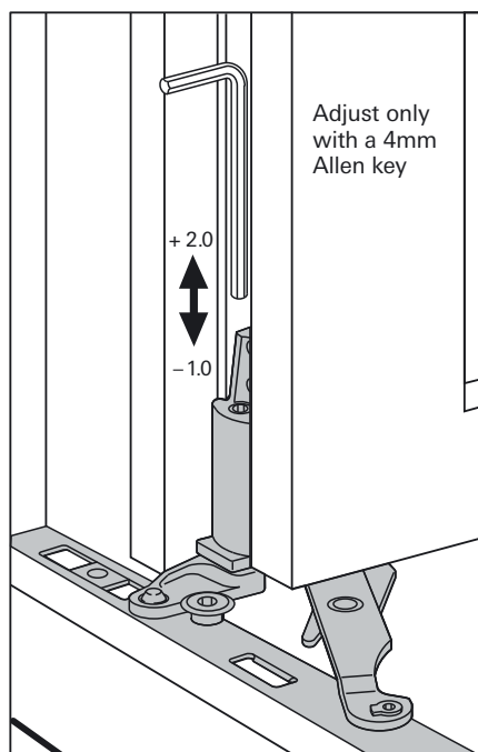
Corner hinge R
